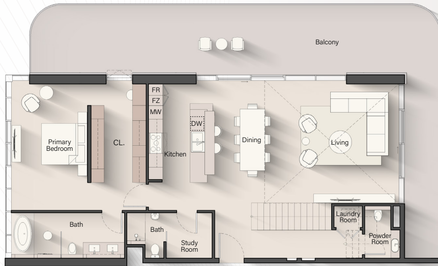
LOWER LEVEL
