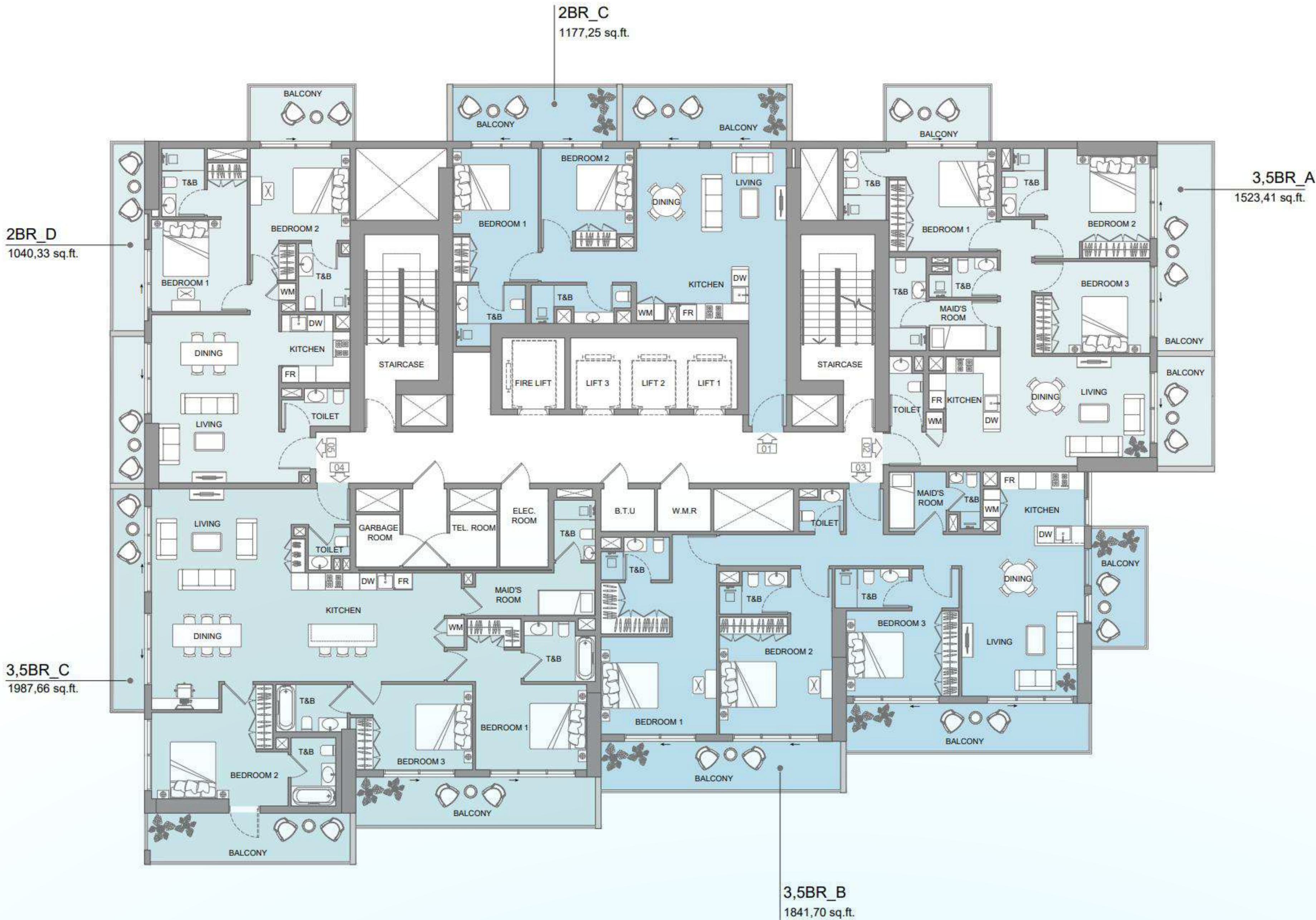
FLOOR PLAN 19TH-20TH
