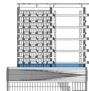
ELEVATION D
