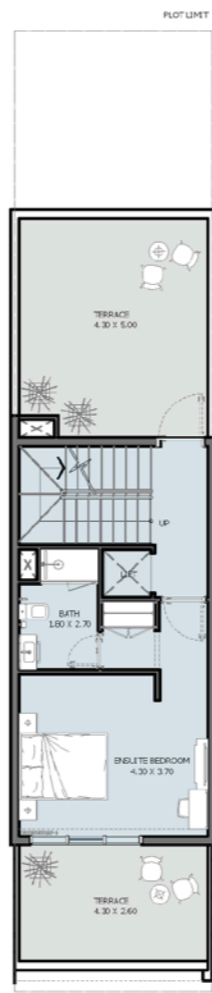
ROOF PLAN
